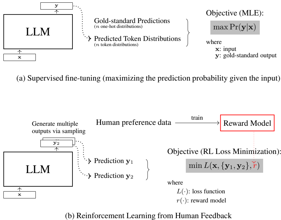
Fig. 4.6: Supervised fine-tuning vs. reinforcement learning from human feedback. In supervised fine-tuning, we optimize the LLM by maximizing the probability of the prediction given the input. In reinforcement learning from human feedback, we first train a reward model on human preference data (on each pair of predictions, evaluators are asked to choose which one they prefer). Then, we use this reward model to supervise the LLM during fine-tuning.
