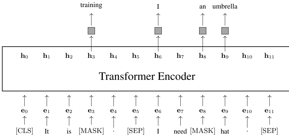
Fig. 1.5: A running example of BERT-style masked language modeling. First, 15% tokens are randomly selected. These selected tokens are then processed in one of three ways: replaced with a [MASK] token (80% of the time), replaced with a random token (10% of the time), or kept unchanged (10% of the time). The model is trained to predict these selected tokens based on the modified sequence. e_i represents the embedding of the token at the position i . Gray boxes represent the Softmax layers.
