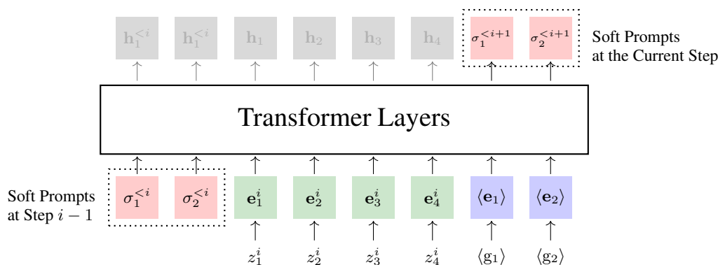
Fig. 3.8: Illustration of compressing a context segment into soft prompts ( \kappa = 2 and m_i = 4 ). The input to the LLM includes the soft prompts from the previous step ( \sigma_1^{<i>i</i>} and \sigma_2^{<i>i</i>} ), the tokens of the segment ( z_1, z_2, z_3 , and z_4 ), and the summary tokens ( \langle g_1 \rangle and \langle g_2 \rangle ). Given these, the LLM operates as usual. We then extract the outputs at the last Transformer layer that correspond to the summary tokens. These outputs can be viewed as the soft prompts that accumulated up to this segment.
